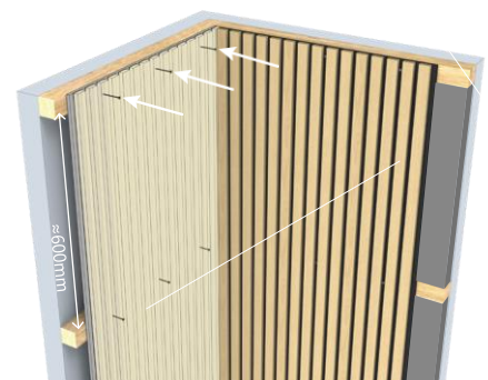
c. Install fibreglass wool or rock wool between the battens. absorption class: A
